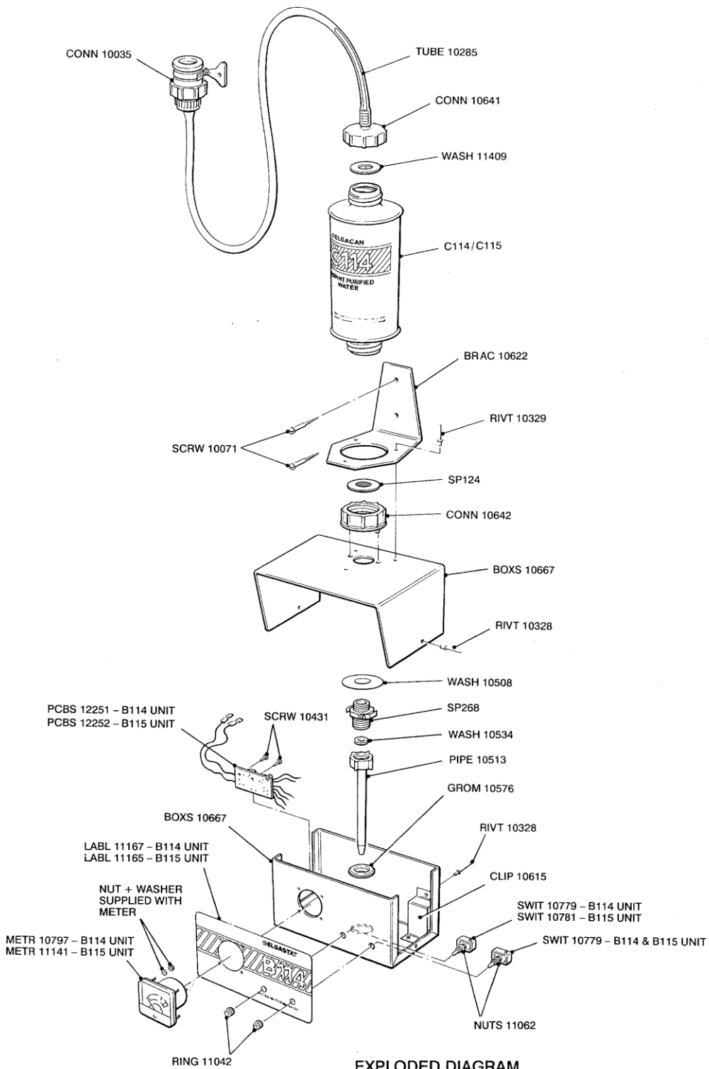
EXPLODED DIAGRAM of ELGASTAT B114 & B115 UNITS
